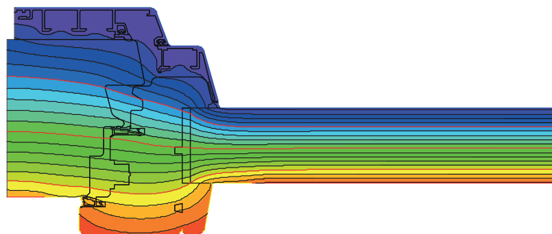
IV92 system harmonious design and rounded lines, suitable for homes with low energy consumption
