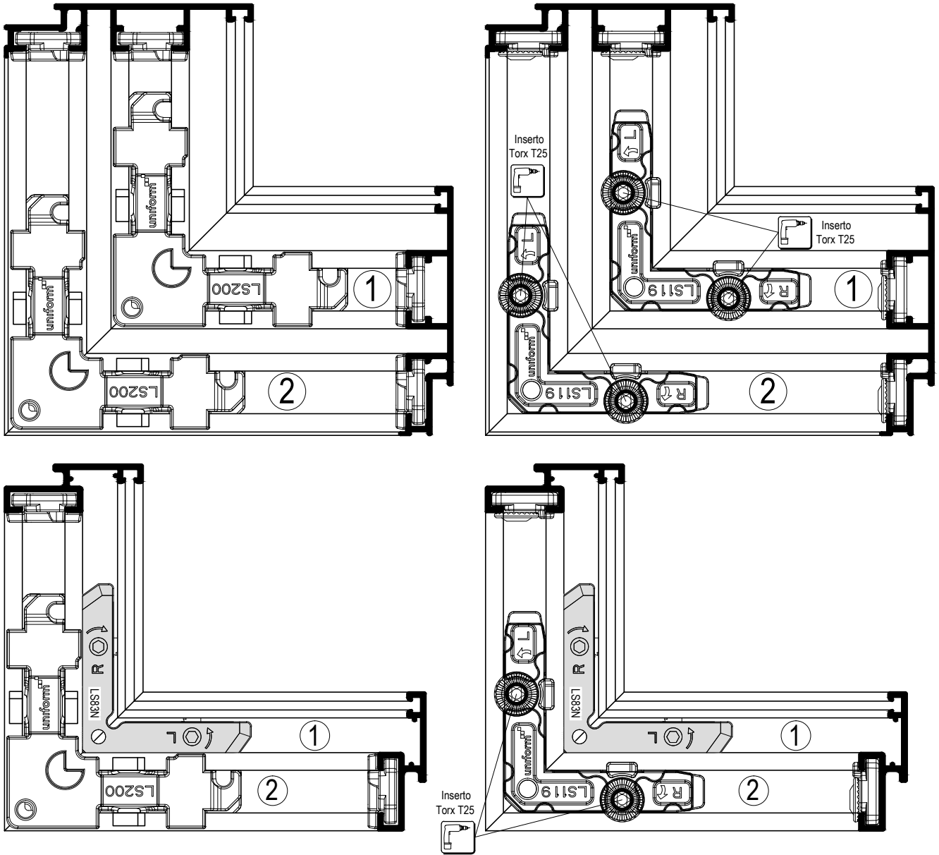
Ante in alluminio sistema Easy-Flat Alumim sash profiles Easy-Flat
