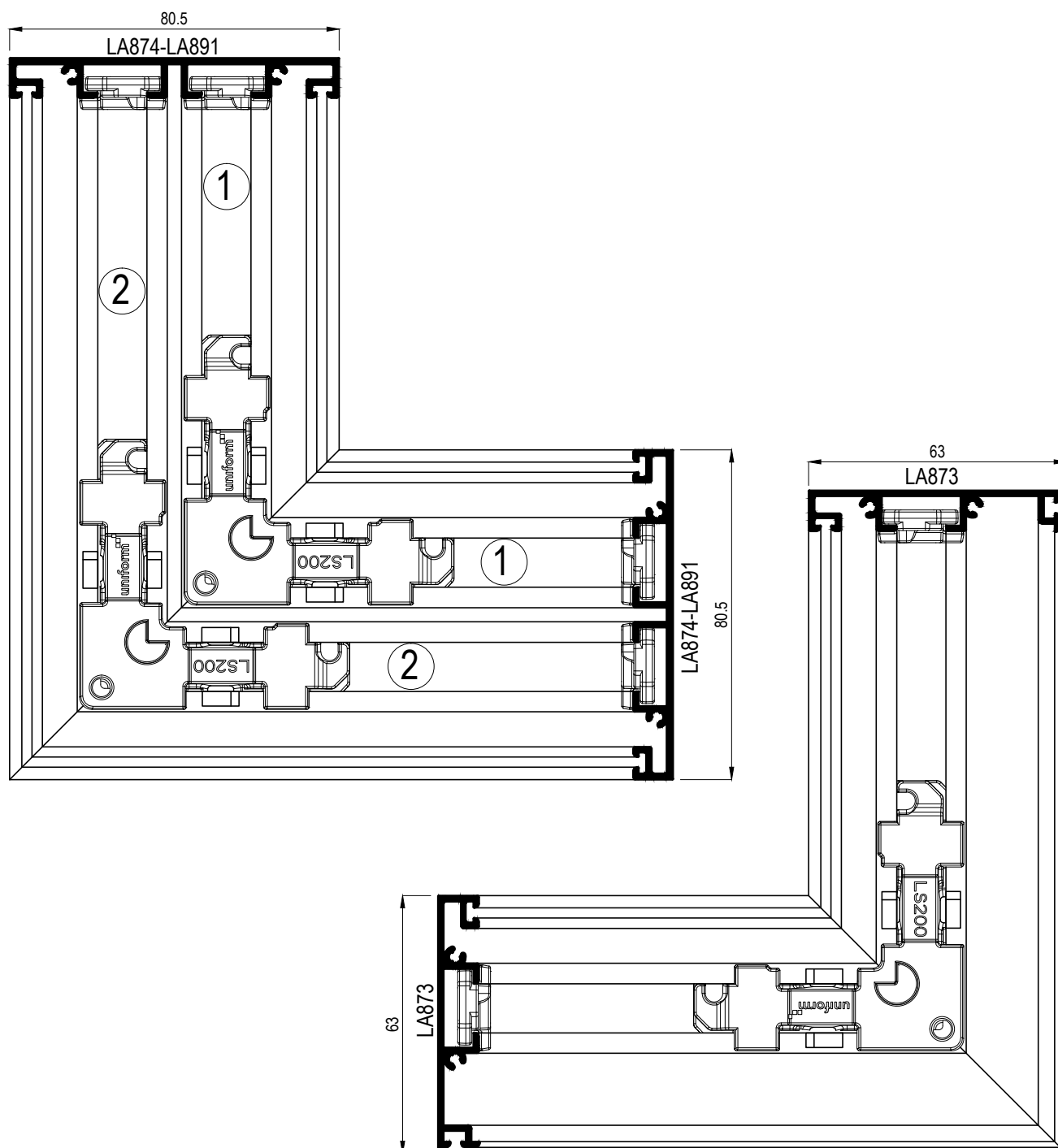
Ante in alluminio sistema Easy-Flat Aluminum sash profiles Easy-Flat system
