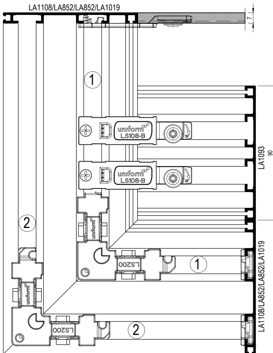
Ante in alluminio sistema Easy-Flat Aluminum sash profiles Easy-Flat system
