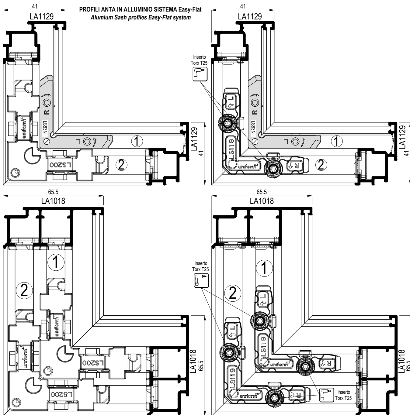
Ante in alluminio sistema Easy-Flat/ Alumium sash profiles Easy-Flat system
