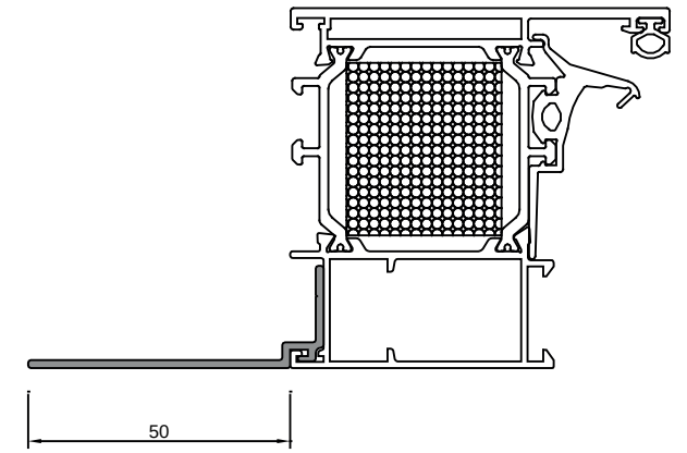
Z-frame, with stop block leaf, 50 mm available
