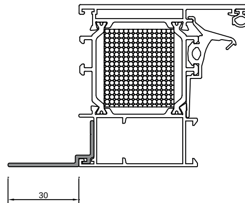
Z-frame, with stop block leaf, 30 mm available
