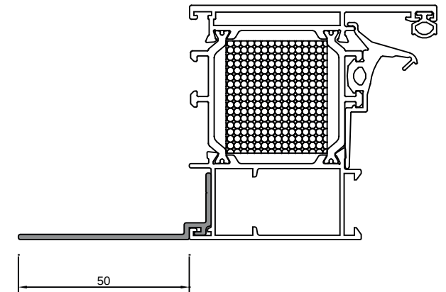
Z-frame, with stop block leaf, 50 mm available
